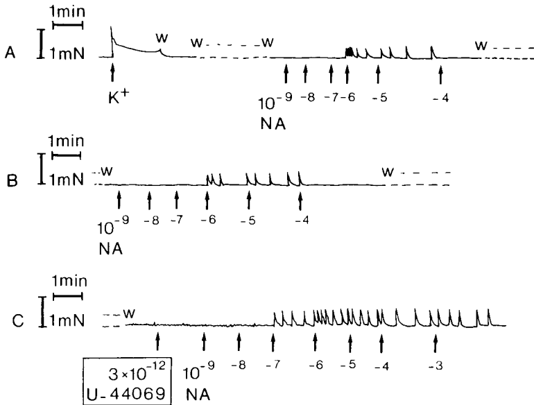
Fig. 5. Tracings obtained from the same lymphatic segment presented in a chronological order (A-C). In A and B, noradrenaline (NA) 10^{-6} M induced phasic contractions. In C, when U-44069 3 \times 10^{-12} M was added before noradrenaline, the phasic contractions occurred at a lower concentration of noradrenaline ( 10^{-7} M). Between the different cumulative additions of noradrenaline several wash out (W) with fresh Krebs buffer solution were made. K + indicates the previous potassium (124mM)-induced contraction. The concentrations of noradrenaline above 10^{-9} M are given as log noradrenaline concentration (in mM).
